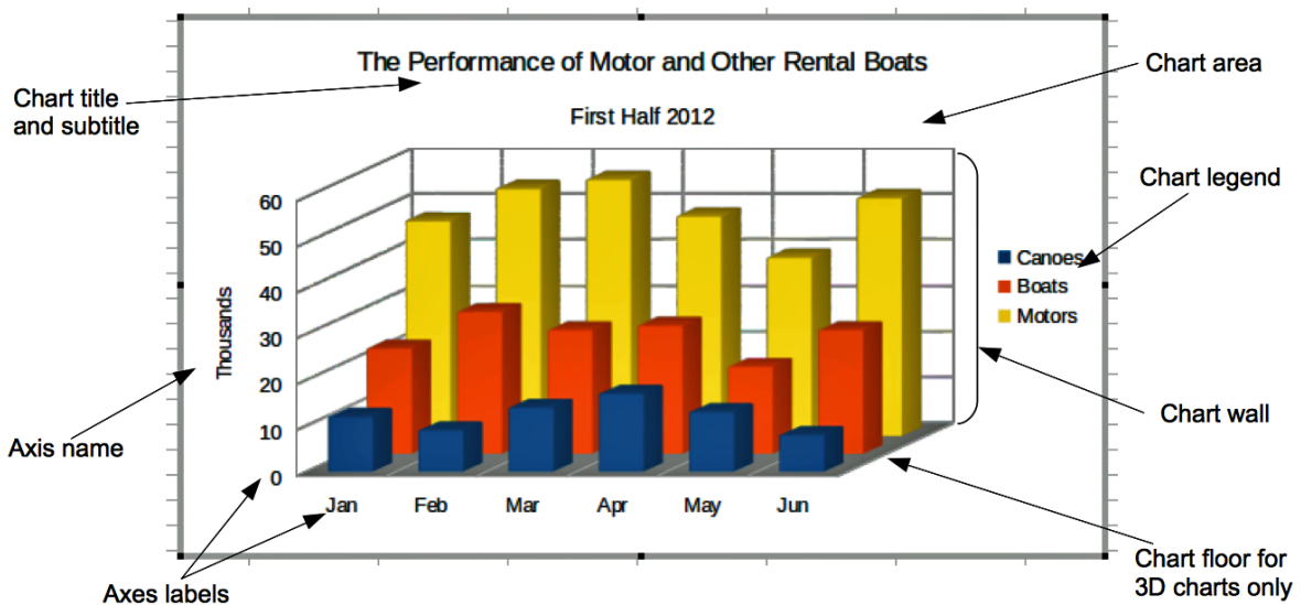
Figure 63: Chart elements
