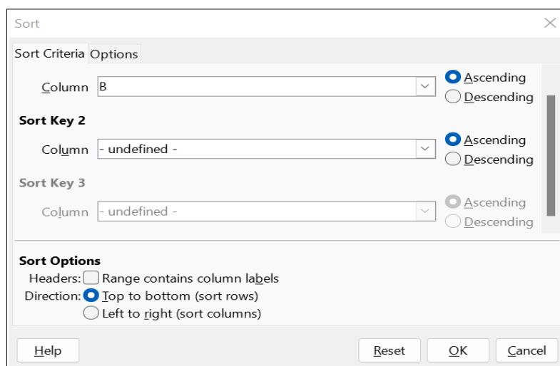
Figure 489: Sort dialog
