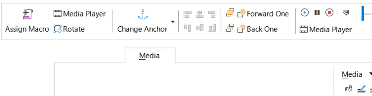
Figure 567: Media tab
