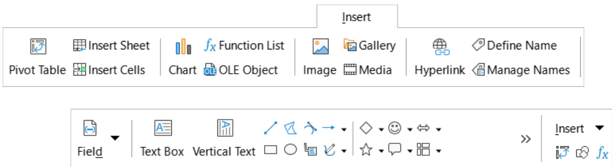
Figure 540: Insert tab
