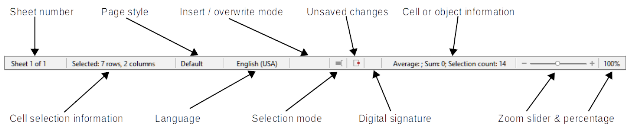
Figure 7: Status Bar
