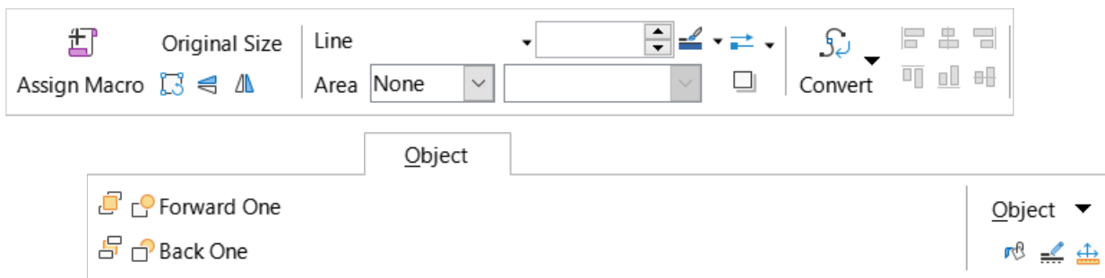
Figure 569: Object tab
