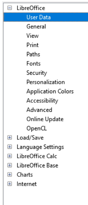
Figure 496: LibreOffice options
