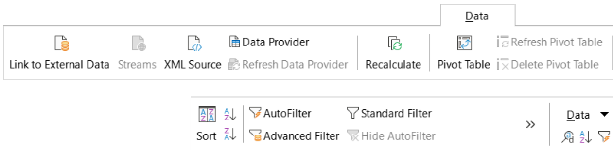
Figure 546: Data tab
