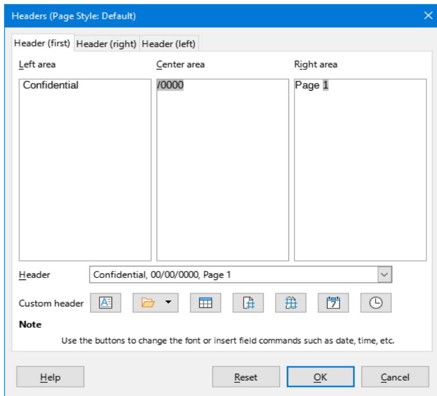
Figure 232: Header dialog
