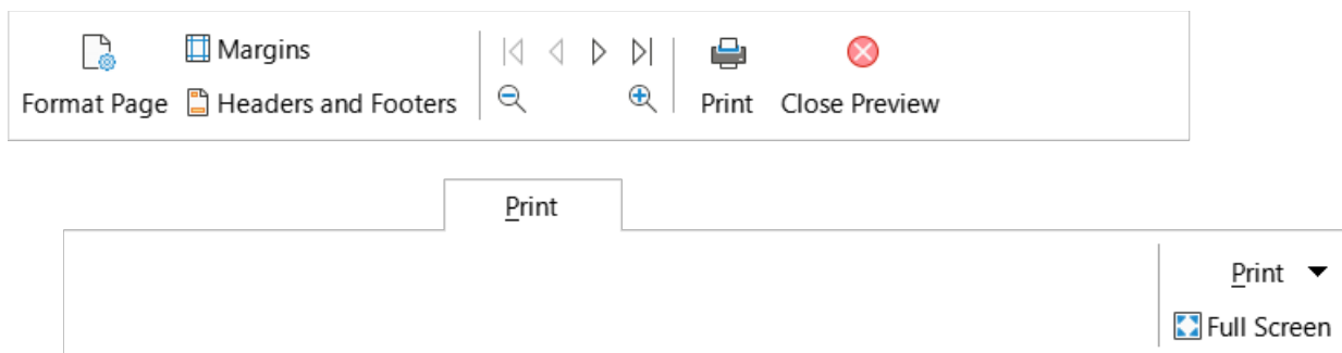
Figure 571: Print tab
