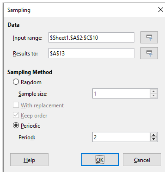
Figure 358: Sampling dialog
