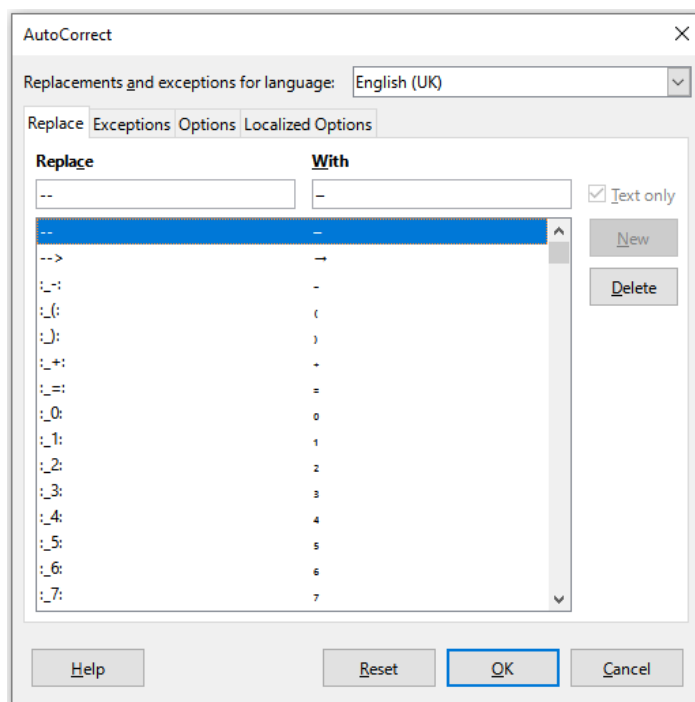
Figure 29: AutoCorrect dialog
