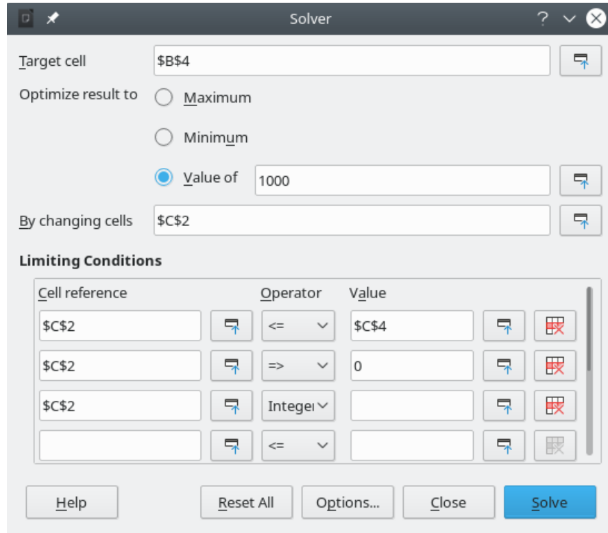
Figure 352: Solver dialog
