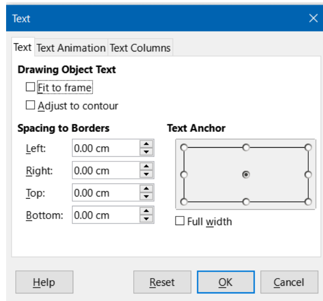
Figure 208: Text dialog
