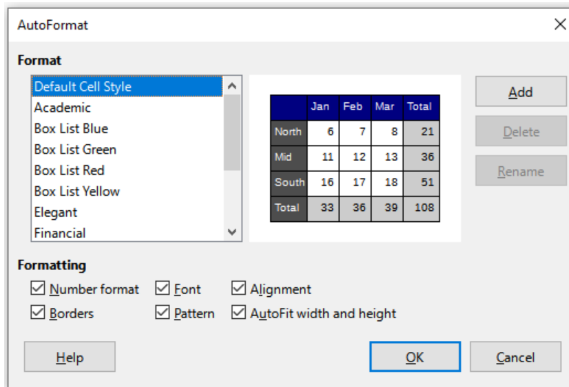
Figure 158: AutoFormat dialog
