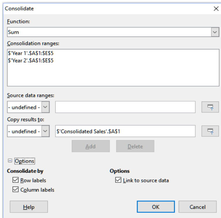
Figure 325: Consolidate dialog
