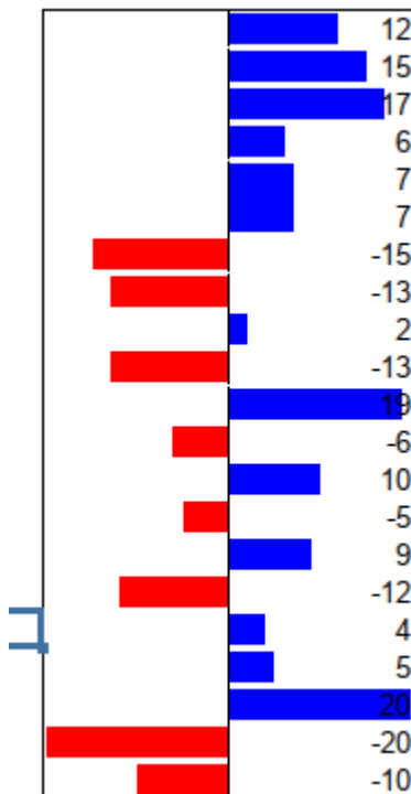
Figure 165: Data bars
