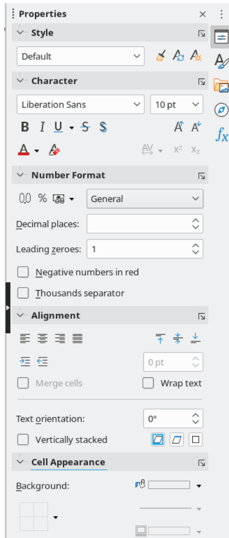
Figure 8: Sidebar
