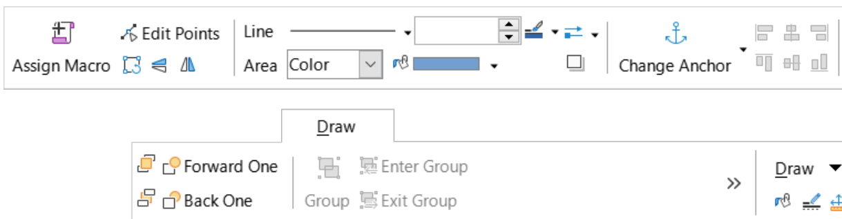
Figure 559: Draw tab
