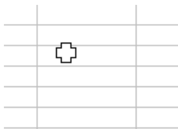
Figure 508: Themed cursor
