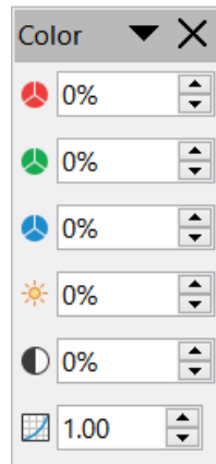
Figure 206: Color toolbar
