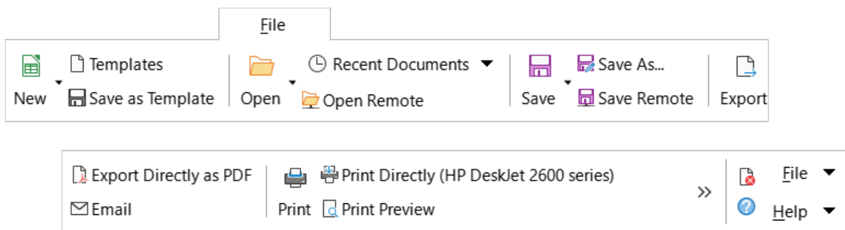
Figure 534: File tab
