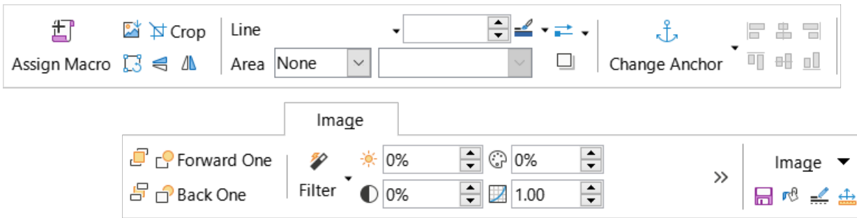
Figure 564: Image tab
