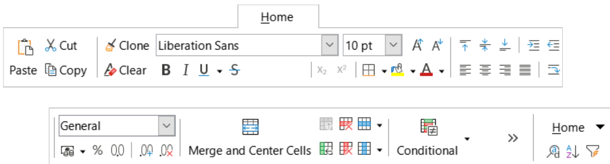
Figure 537: Home tab
