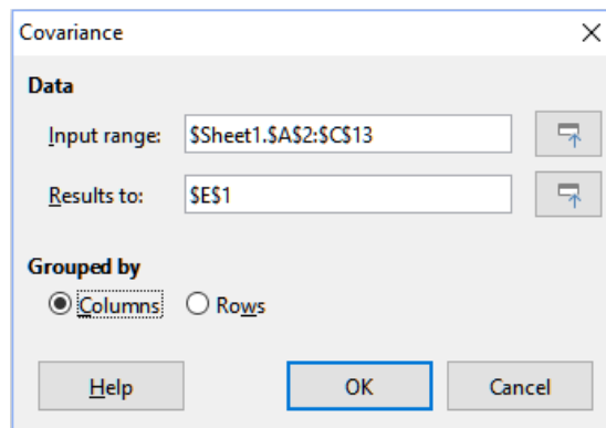
Figure 367: Covariance dialog
