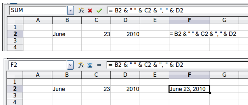
Figure 244: Text concatenation
