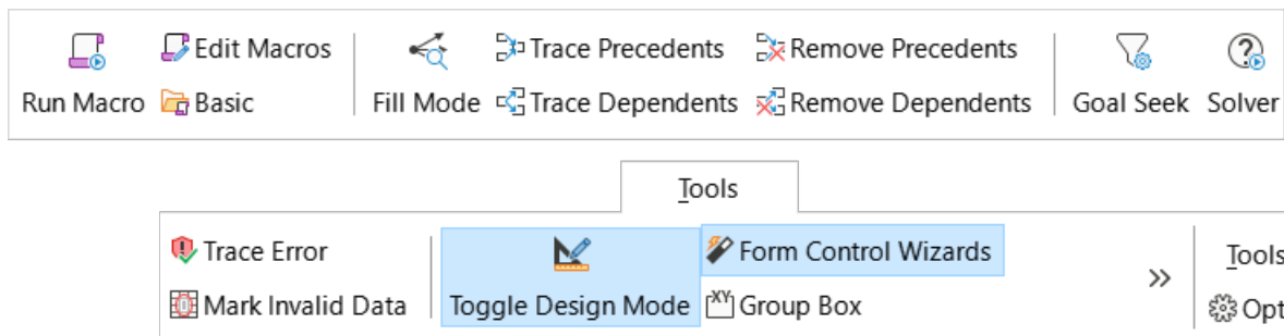
Figure 556: Tools tab
