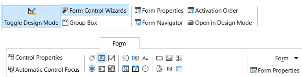
Figure 562: Form tab
