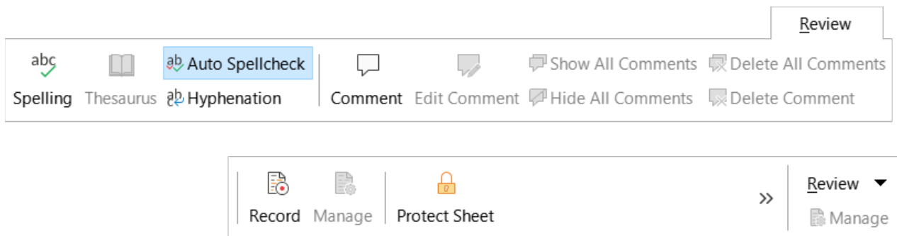
Figure 549: Review tab
