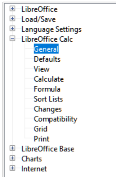
Figure 504: Calc options
