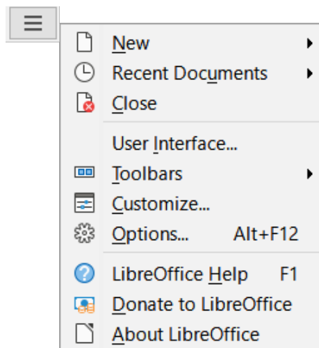
Figure 533: Quick menu
