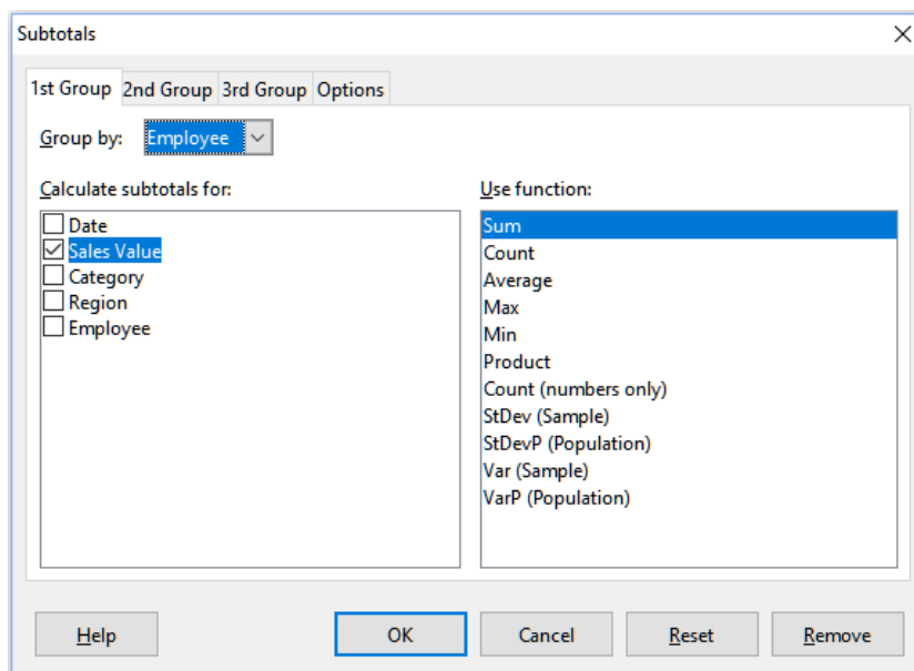
Figure 333: Subtotals dialog
