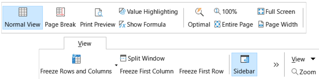
Figure 552: View tab
