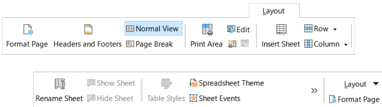
Figure 543: Layout tab
