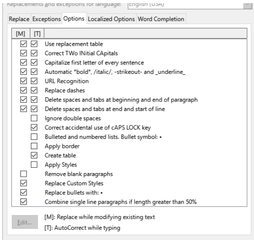
Figure 94: Autoformatting choices on the Options tab
