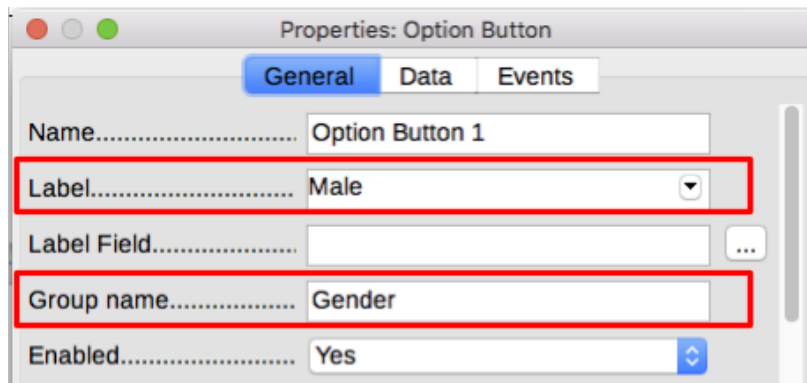
Figure 421: Specifying label and group names for an option button
