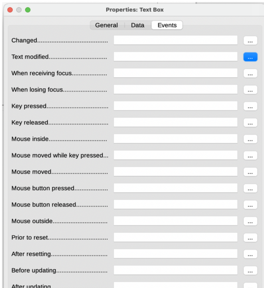
Figure 434: Control properties, Events tab
