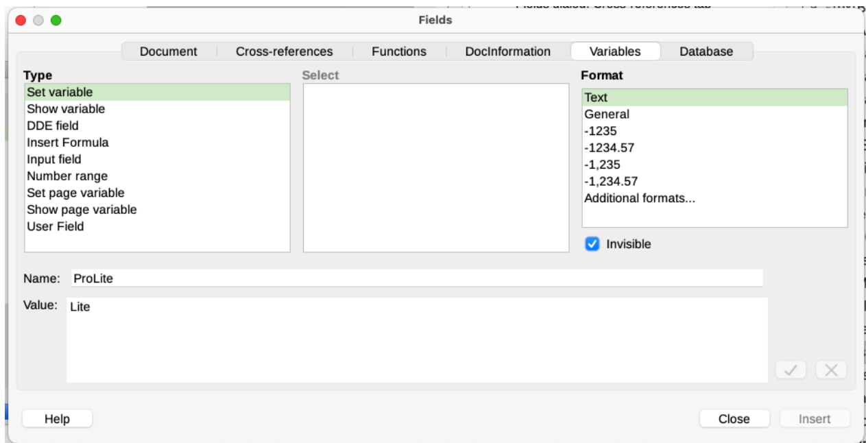
Figure 407: Defining a variable to use with conditional content
