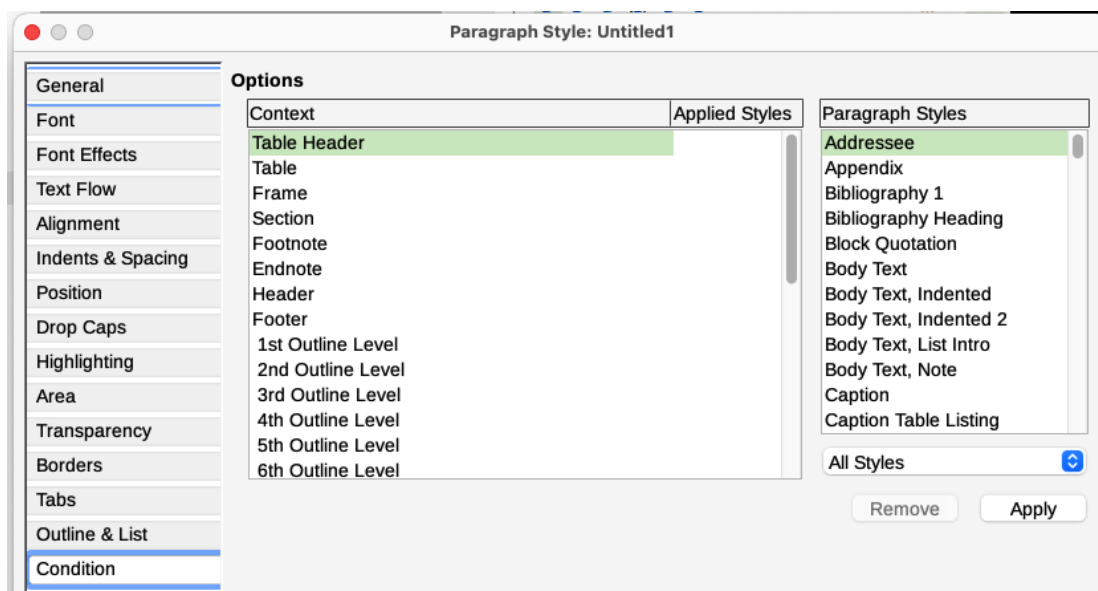
Figure 223: Condition tab for paragraph styles
